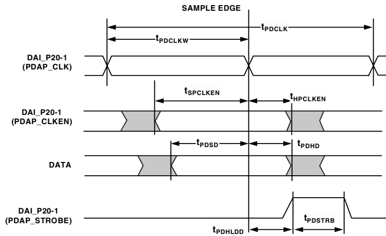
Figure 19. PDAP Timing
