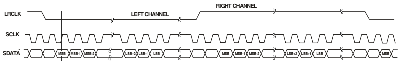
Figure 23. I 2 S-Justified Mode
